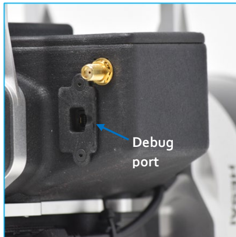
Figure 40. Debug port.
