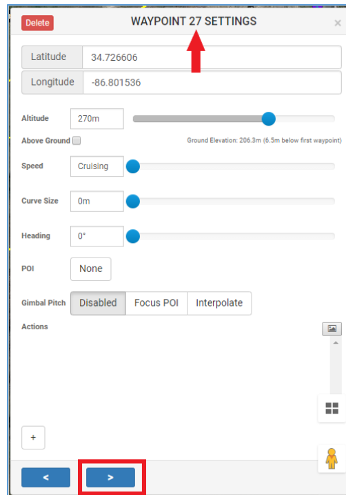
Figure 24 – Waypoint Settings
